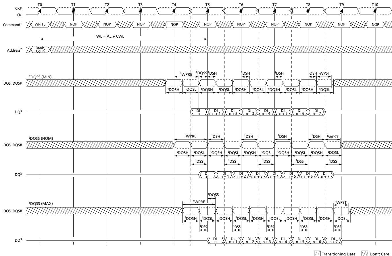
Figure 84: WRITE Burst
