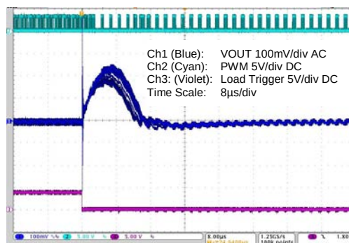
Figure 5.5 15 to 5A Load Step – Max. Capacitance
