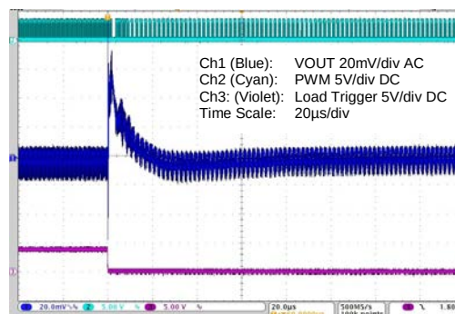
Figure 5.15 15 to 5A Load Step – Max. Capacitance
