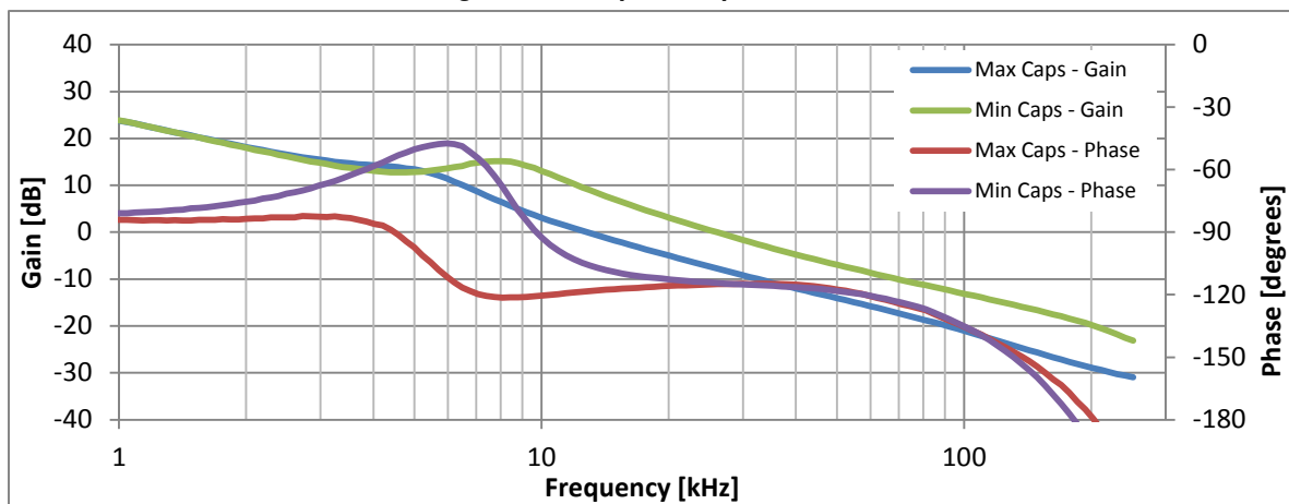
Figure 5.16 Open Loop Bode Plots
