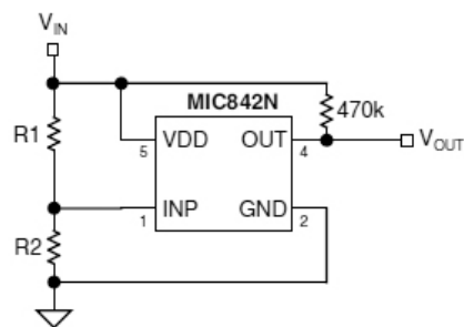
Figure 3. MIC842 Example Circuit
