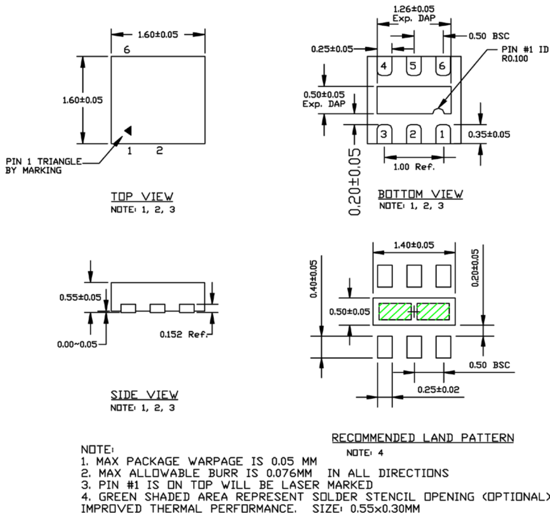
6-Pin 1.6mm × 1.6mm TDFN (MT)
