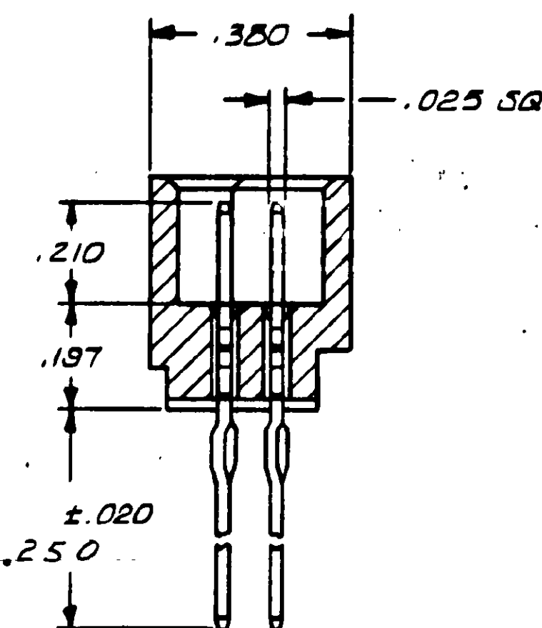
SECTION X-X
