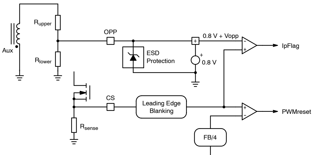
Figure 28. The Internal OPP Circuitry Implemented on NCP1336
