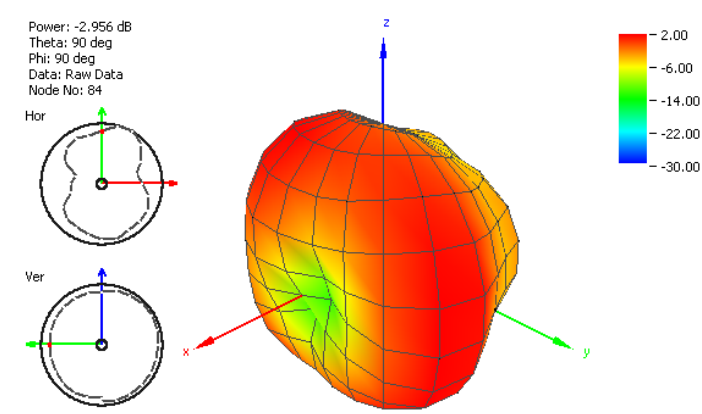
Figure 25. Radiation Pattern at 1850 MHz of FXUB70 Port 2.
