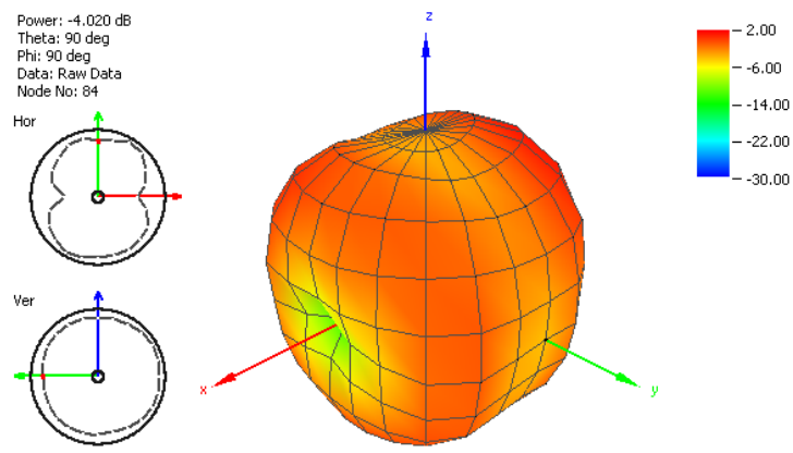
Figure 21. Radiation Pattern at 1575 MHz of FXUB70 Port 2.
