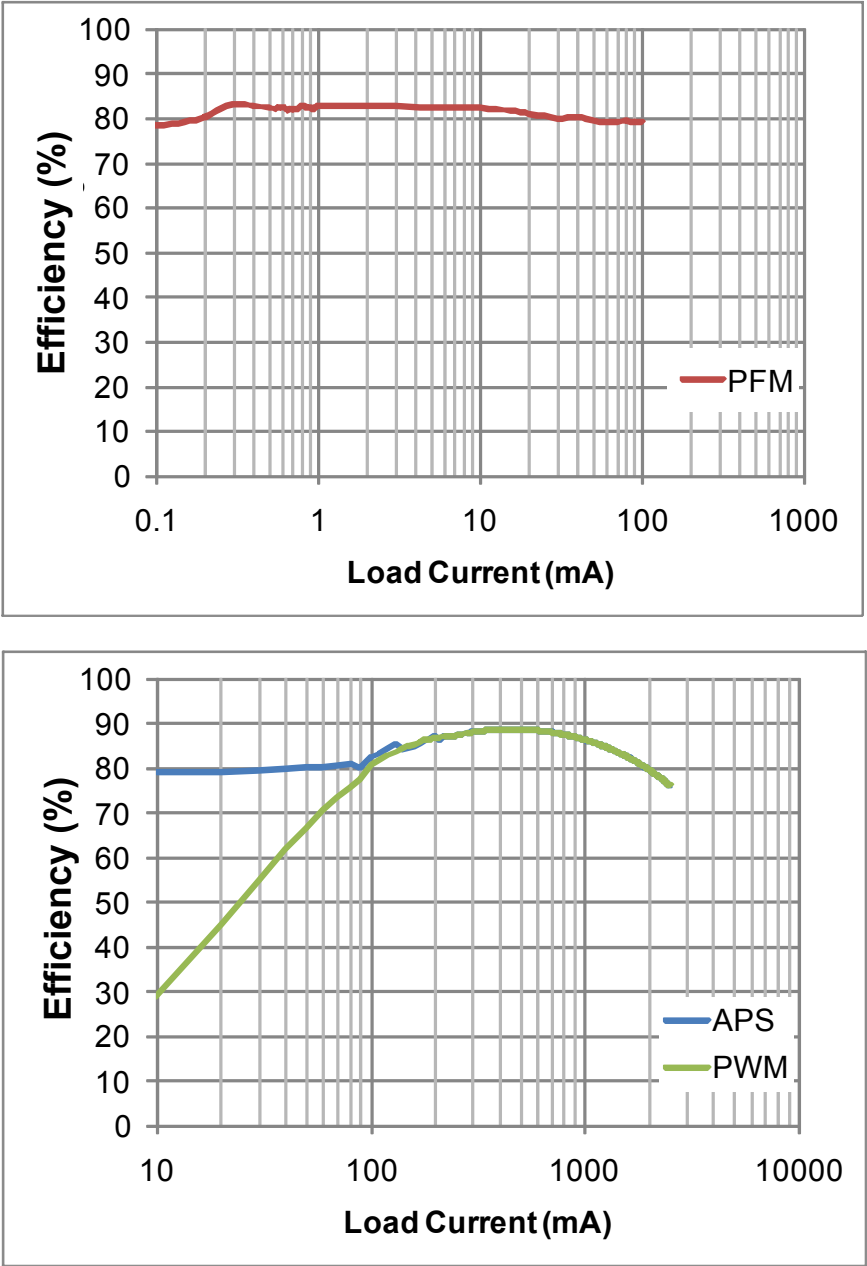
Figure 24. SW3AB Efficiency Waveforms: V_{IN} = 4.2\text{ V} ; V_{OUT} = 1.5\text{ V} ; Consumer Version
