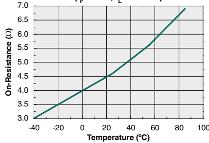
On-Resistance vs. Temperature DC-Only Configuration ( I_F=0\text{mA} , I_L=100\text{mA} )
