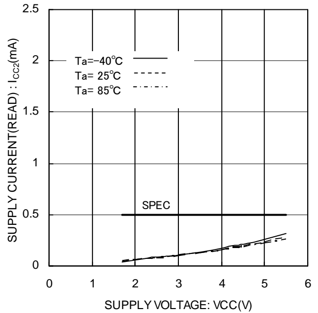
Figure 15. Supply current (READ) I_{CC2} (READ, f_{SK}=1\text{MHz} )
