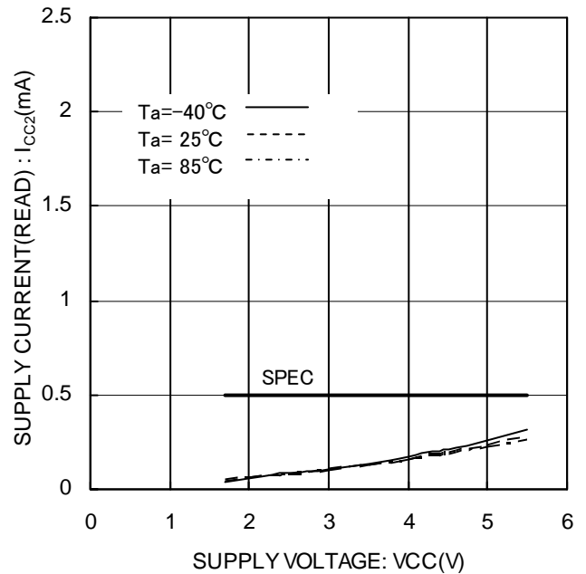
Figure 15. Supply current (READ) I_{CC2}(READ, f_{SK}=1MHz)
