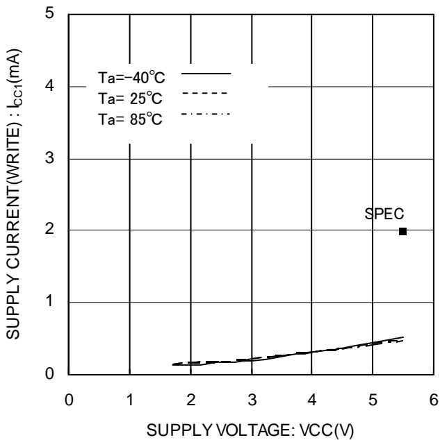
Figure 14. Supply current (WRITE) I_{CC1} (WRITE, f_{SK}=3\text{MHz} )
