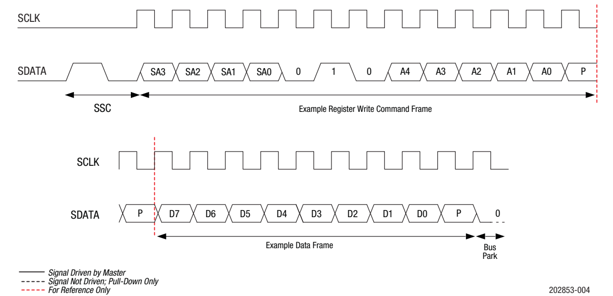
Figure 4. Register Write Command Timing Diagram
