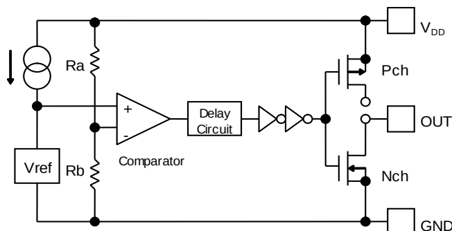
Figure 12. Block Diagram
