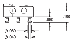
TERMINAL STYLE 1 SINGLE SOLDER TURRET
