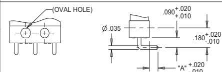
TERMINAL STYLE 9 RIGHT ANGLE, OPPOSITE OF 7
