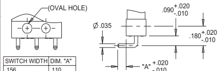
TERMINAL STYLE 7 RIGHT ANGLE PRINTED CIRCUIT PIN
