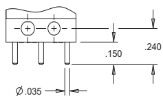
TERMINAL STYLE 4 PRINTED CIRCUIT PIN 0.150" LONG
