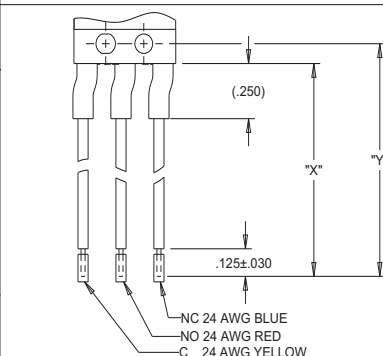
TERMINAL STYLE 9 RIGHT ANGLE, OPPOSITE OF 7
