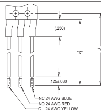
TERMINAL STYLE 9 RIGHT ANGLE, OPPOSITE OF 7
