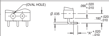
TERMINAL STYLE 9 RIGHT ANGLE, OPPOSITE OF 7
