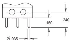
TERMINAL STYLE 4 PRINTED CIRCUIT PIN 0.150" LONG
