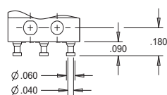
TERMINAL STYLE 1 SINGLE SOLDER TURRET
