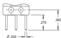
TERMINAL STYLE 5 PRINTED CIRCUIT PIN 0.270" LONG
