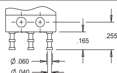
TERMINAL STYLE 2 DOUBLE SOLDER TURRET
