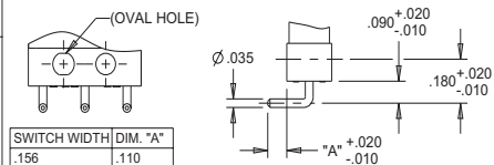
TERMINAL STYLE 7 RIGHT ANGLE PRINTED CIRCUIT PIN
