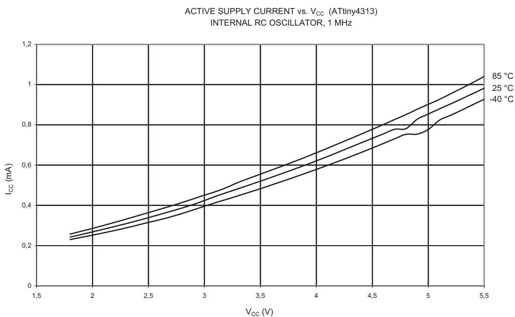
Figure 23-52. Active Supply Current vs. V_{CC} (Internal RC Oscillator, 1 MHz)
