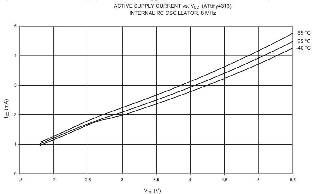
Figure 23-51. Active Supply Current vs. V_{CC} (Internal RC Oscillator, 8 MHz)
