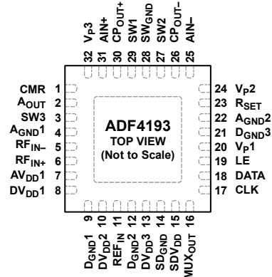
Figure 3. Pin Configuration
