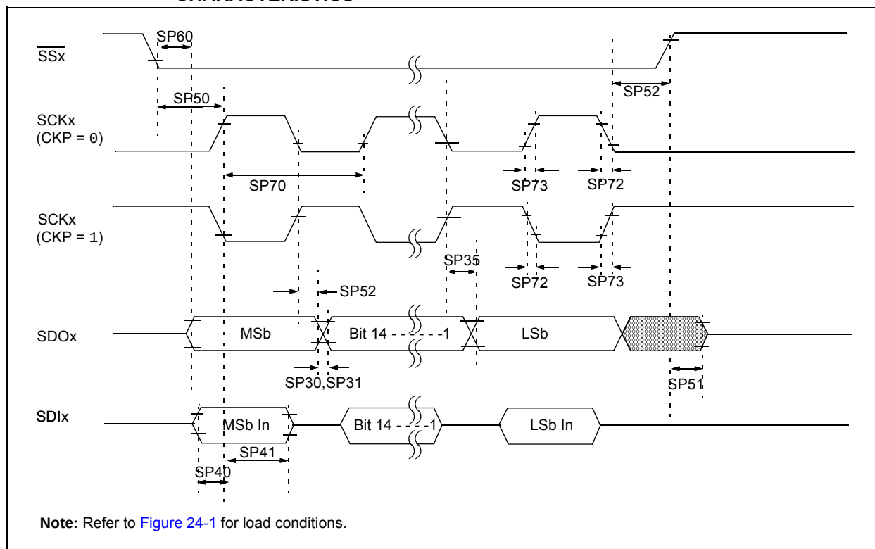
FIGURE 24-14: SPIx SLAVE MODE (FULL-DUPLEX, CKP = 1, CKP = 1, SMP = 0) TIMING CHARACTERISTICS
