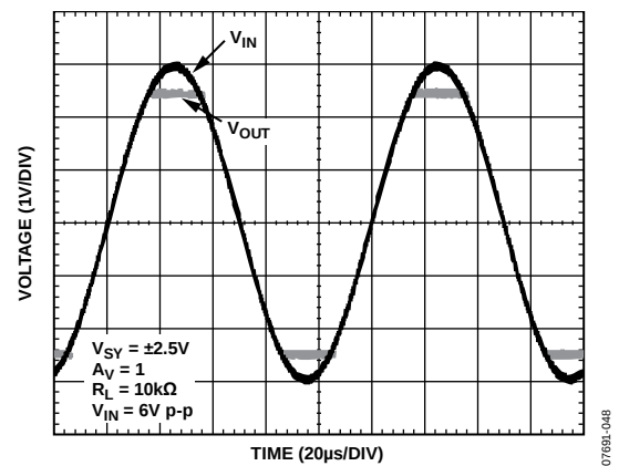
Figure 48. Amplifier, No Phase Reversal
