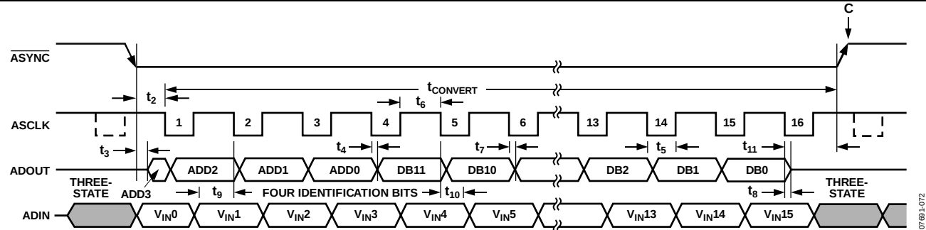
Figure 72. Writing to Shadow Register Timing Diagram
