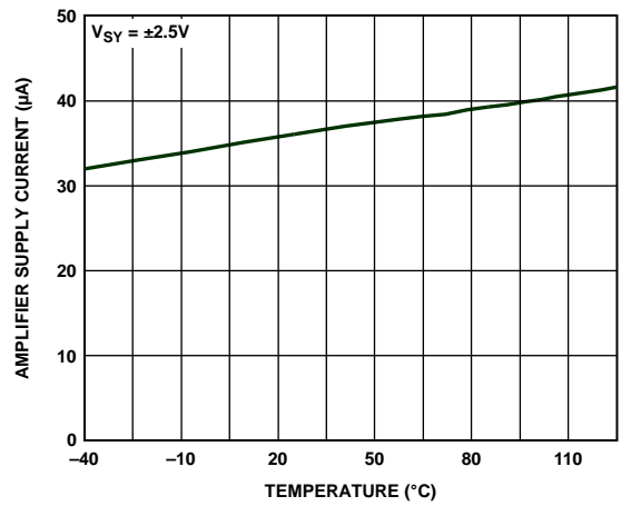
Figure 35. Amplifier Supply Current vs. Temperature
