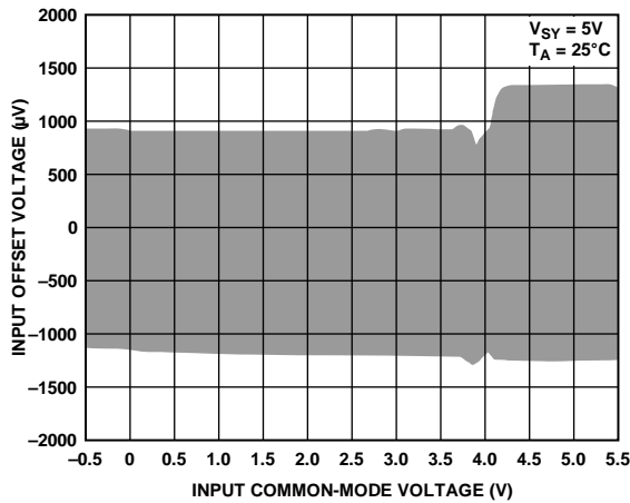
Figure 33. Amplifier Input Offset Voltage vs. Input Common-Mode Voltage
