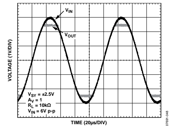
Figure 48. Amplifier, No Phase Reversal
