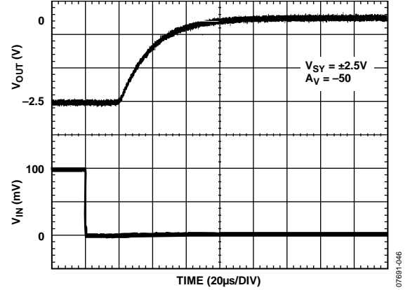
Figure 46. Amplifier Positive Overload Recovery
