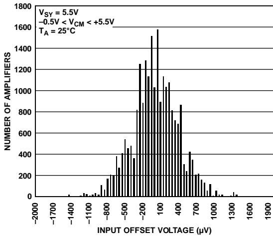
Figure 31. Amplifier Input Offset Voltage Distribution
