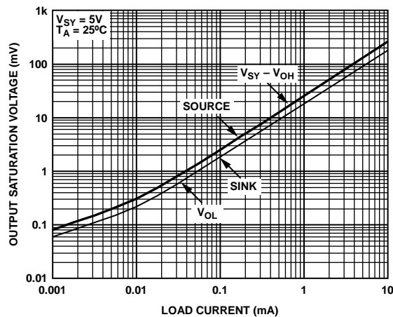
Figure 36. Amplifier Output Saturation Voltage vs. Load Current
