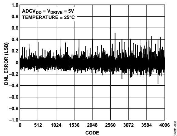
Figure 30. ADC Typical DNL
