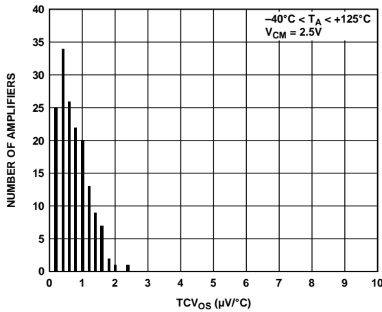
Figure 32. Amplifier Input Offset Voltage Drift Distribution
