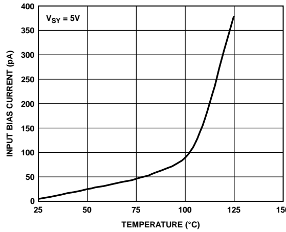
Figure 34. Amplifier Input Bias Current vs. Temperature
