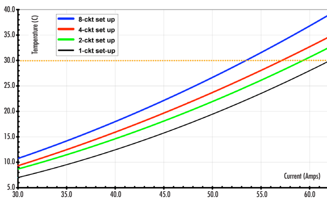
Temperature Rise vs. Current per EIA-364-70
