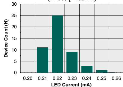
Typical I_F for Switch Operation (N=50, I_L=100\text{mA} )
