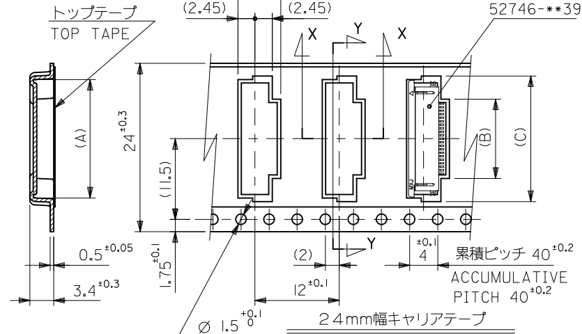
SECT.Y-Y
