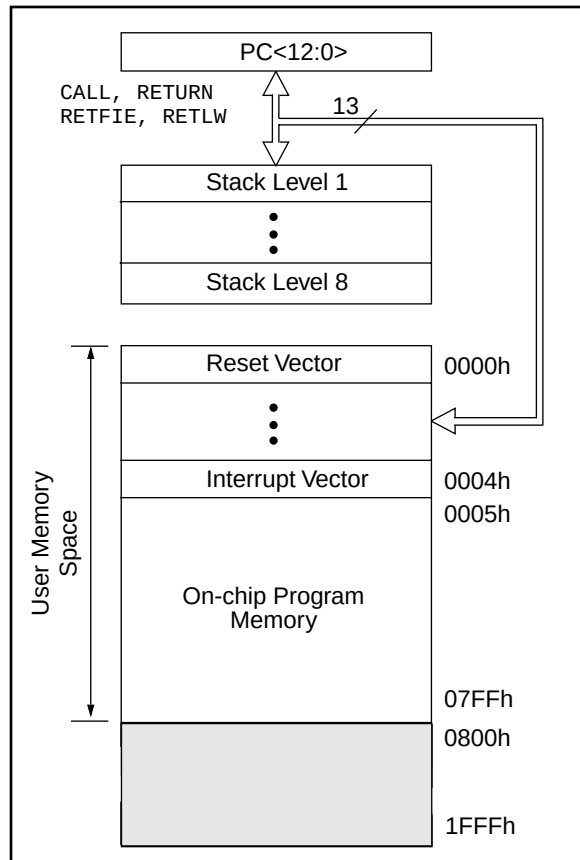
FIGURE 4-1: PIC16C72 PROGRAM MEMORY MAP AND STACK
