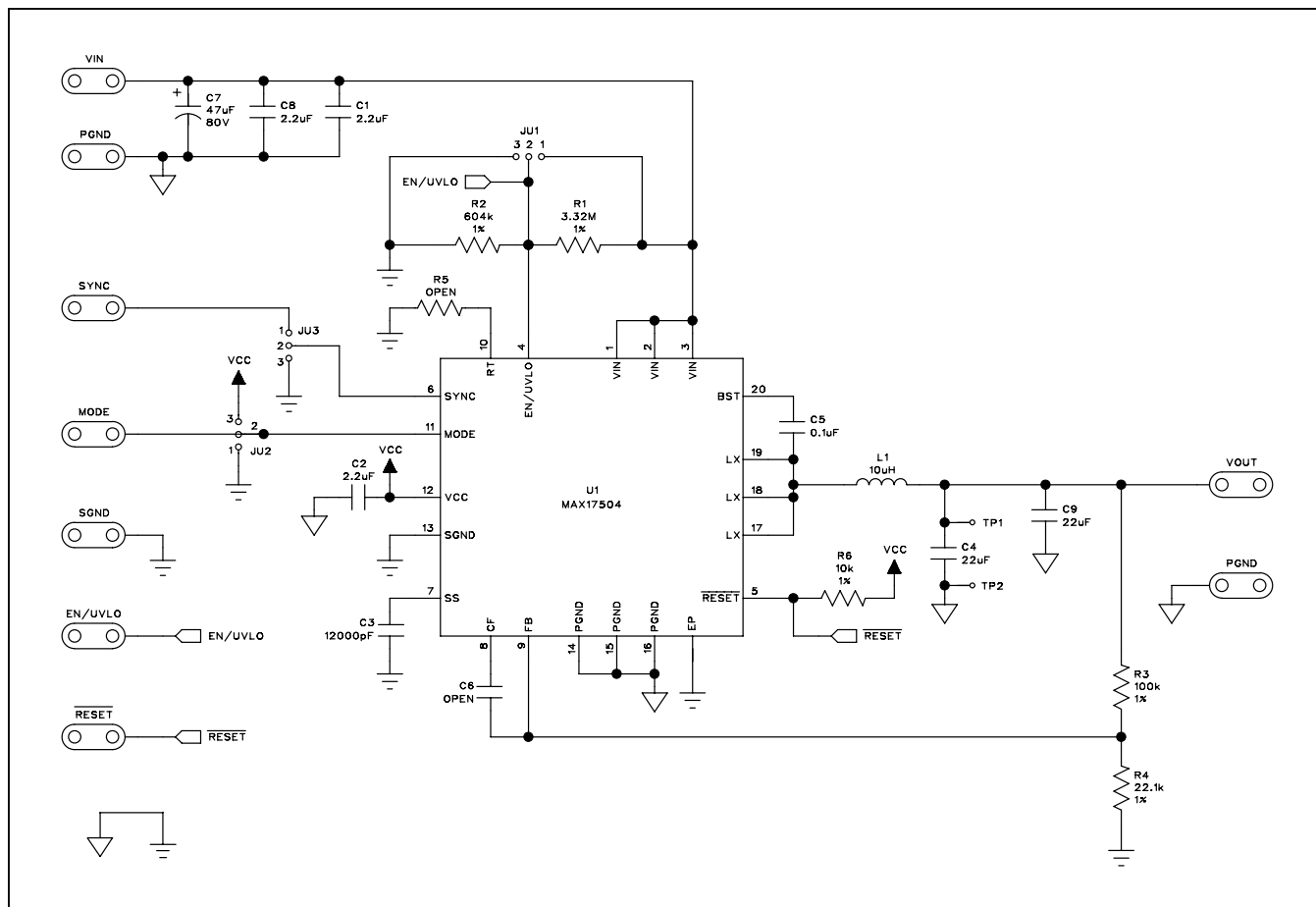
Figure 11. MAX17504 5V Output EV Kit Schematic
