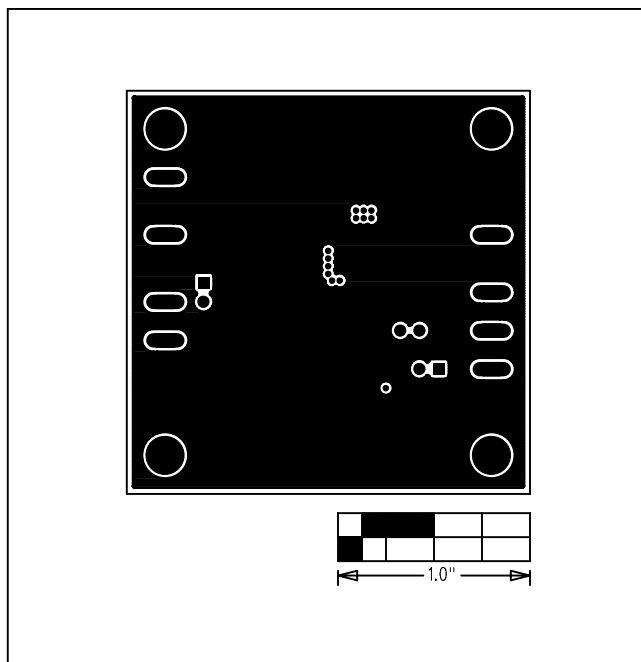
Figure 14. MAX17504 5V Output EV Kit PCB Layout—Inner Layer 1
