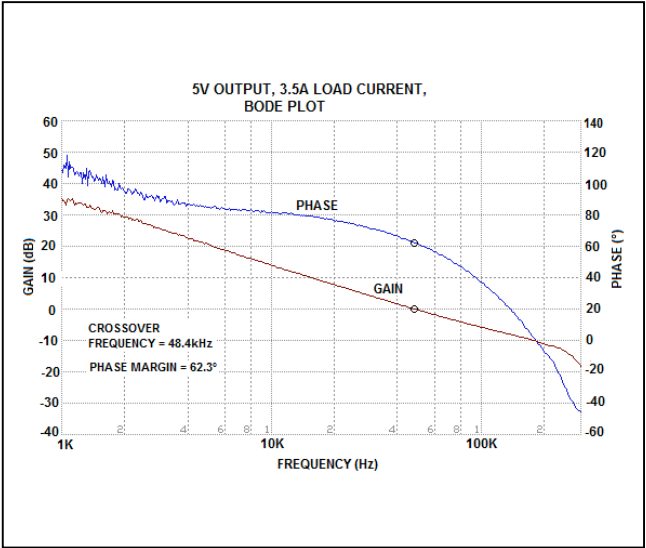
Figure 6. MAX17504 5V Output Full Load Bode Plot ( V_{IN} = 24V )
