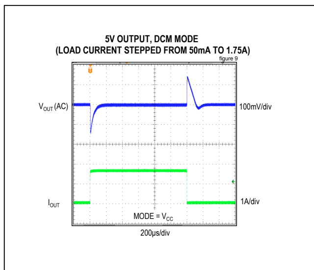
Figure 9. MAX17504 5V Output, 50mA to 1.75A Load Transient (DCM Mode)
