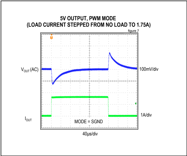
Figure 7. MAX17504 5V Output, No Load to 1.75A Load Transient (PWM Mode)
