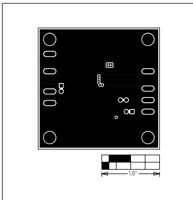
Figure 15. MAX17504 5V Output EV Kit PCB Layout—Inner Layer 2
