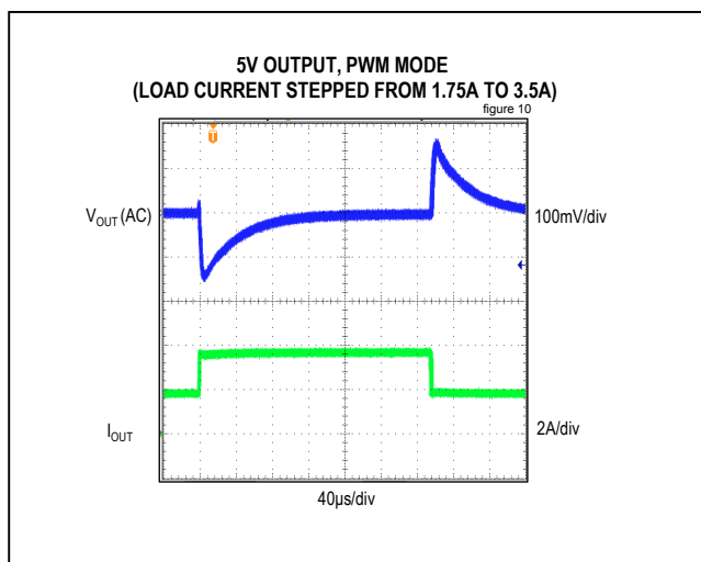
Figure 10. MAX17504 5V Output, 1.75A to 3.5A Load Transient
