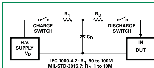
Figure 1: Electrostatic Discharge Test
