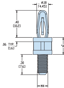
BAYONET SNAP LOCK 10,2 / M4 MALE THREAD
