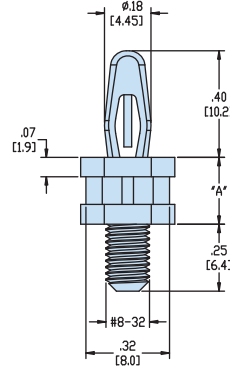
BAYONET SNAP LOCK 10,2 / 8-32 MALE THREAD
