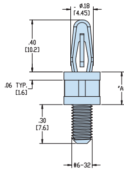
BAYONET SNAP LOCK 10,2 / 6-32 MALE THREAD
