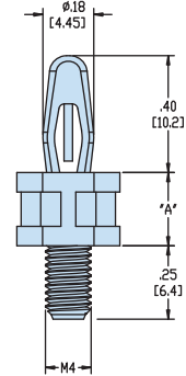
BAYONET SNAP LOCK 10,2 / M4 MALE THREAD
