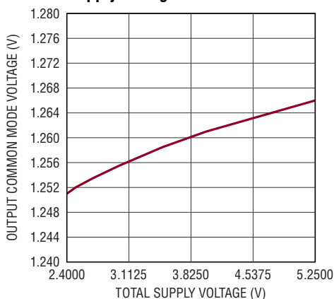
Output Common Mode Voltage vs Supply Voltage
