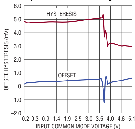
Input Offset, Hysteresis vs Input Common Mode Voltage
