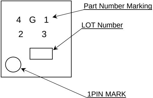
TSSOP-B8J(TOP VIEW)
