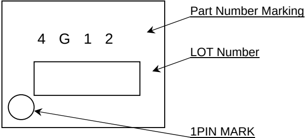
SOP8(TOP VIEW)
