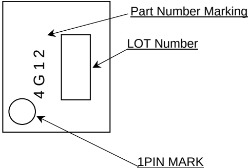
TSSOP-B8(TOP VIEW)
