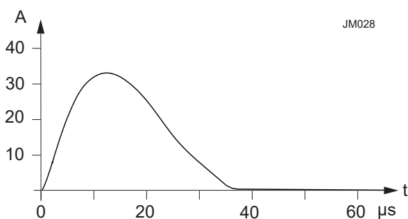
Fig. 3 Inrush current at V_{i \text{ nom}} , P_{o \text{ nom}} versus time (110IMY70-24-24-8). Source impedance according to ETS 300132-2: L = 10 \mu\text{H} , R = 1.5 \Omega .
