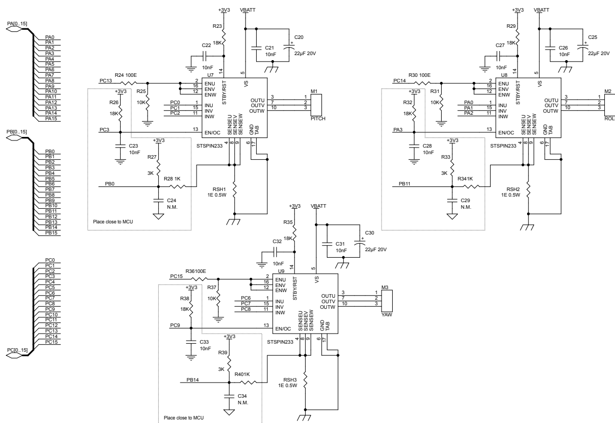
Figure 3. STEVAL-GMBL01V1 schematic – motor control
