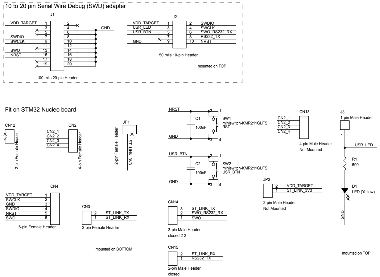
Figure 4. STEVAL-UKI001V1 schematic
