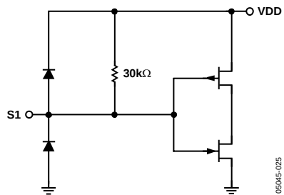
Figure 25. S1 Input
