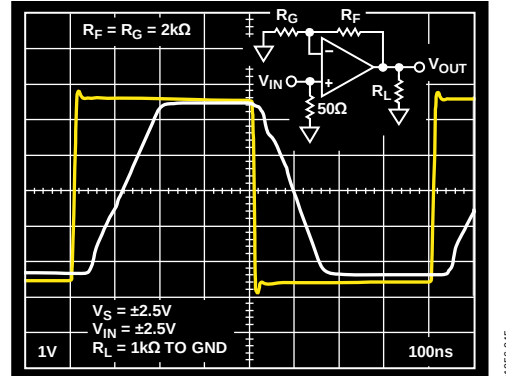
Figure 45. Overdrive Recovery
