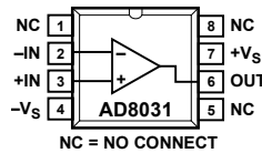
Figure 1. 8-Lead PDIP (N) and SOIC_N (R)
