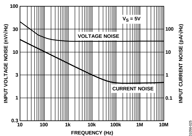
Figure 25. Input Voltage Noise vs. Frequency
