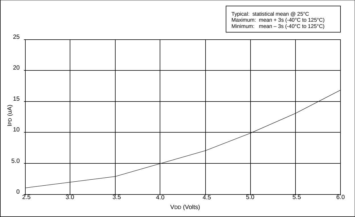
FIGURE 20-2: TYPICAL I PD vs. V DD , WATCHDOG ENABLED (25°C)
