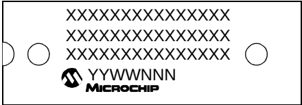
28-Lead PDIP (.600")
