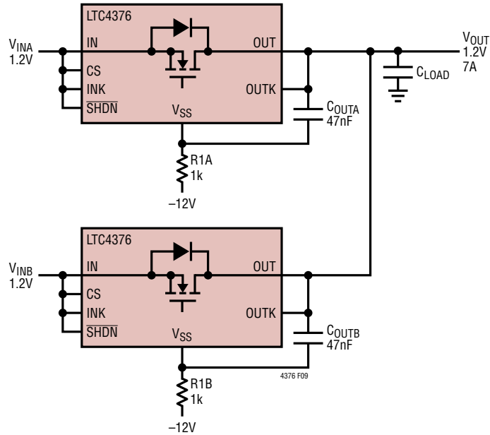
Figure 9. 1.2V Diode-OR
