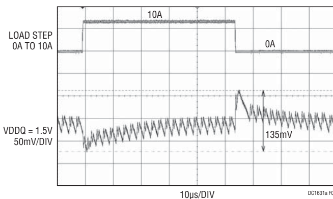
Figure 3. Load Step Response of the VDDQ on the DC1631A at V_{IN} = 12V . C_{OUT} = 2 \times \text{Sanyo 2R5TPE330M9} \parallel 1 \times 100\mu F \text{ X5R } 6.3V \text{ 1206} , L = 0.47\mu H , f_{SW} = 400kHz
