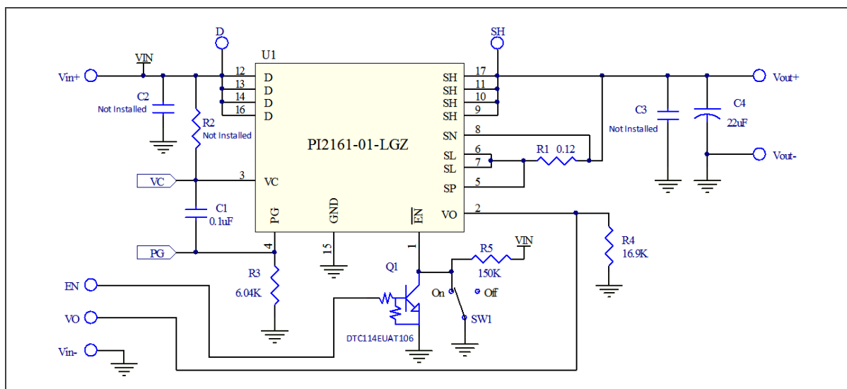
Figure 2: PI2161-EVAL1 Evaluation Board schematic.
