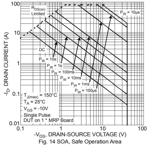
Fig. 14 SOA, Safe Operation Area
