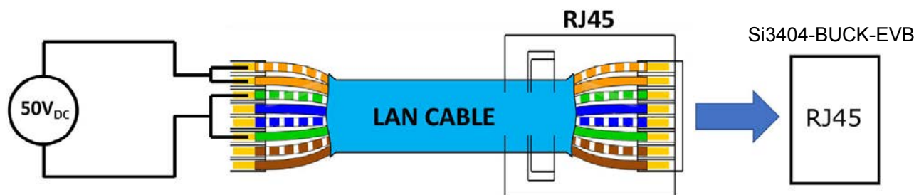
Figure 2.2. Midspan Connection using Laboratory Power Supply
