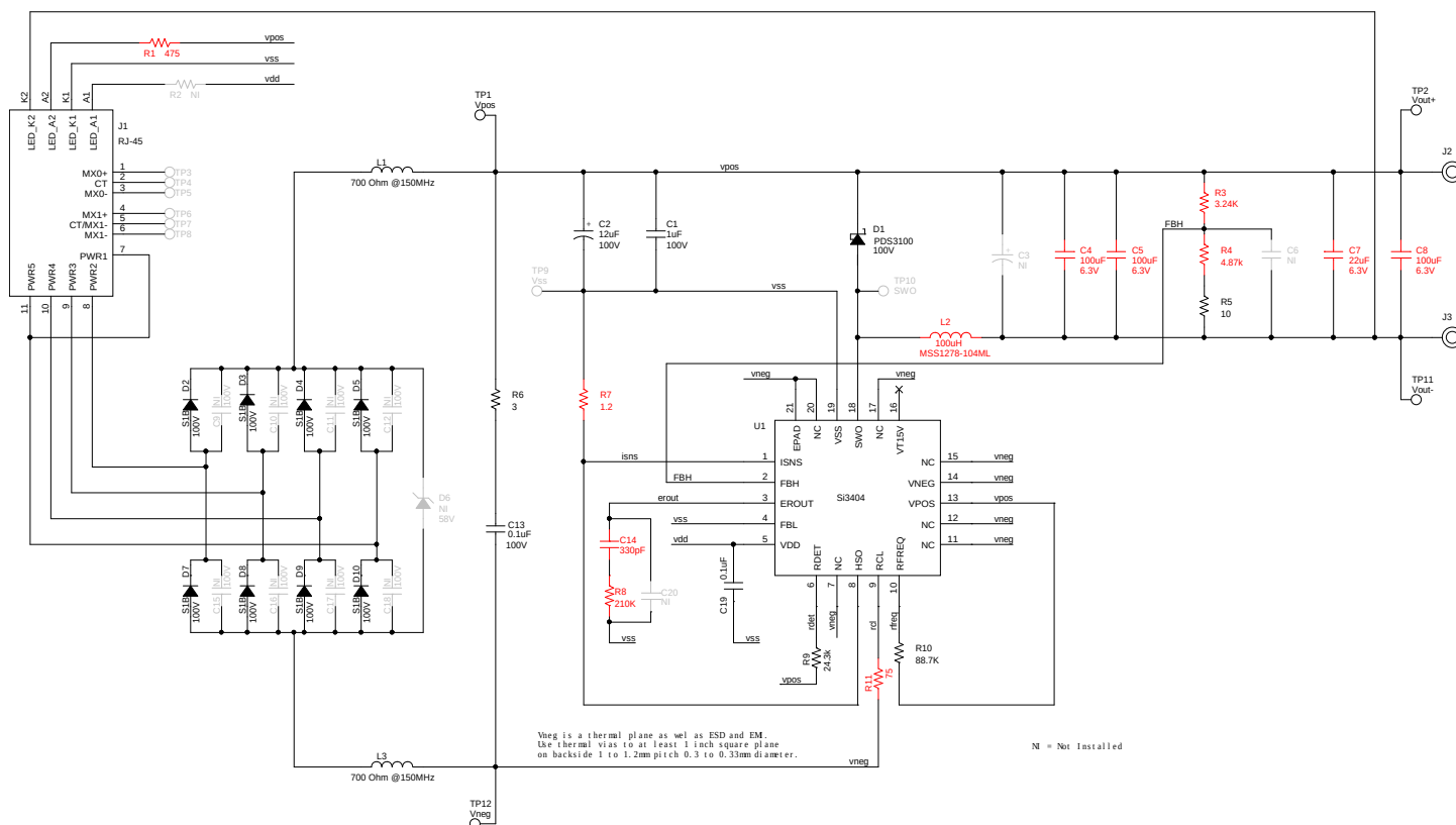
Figure 3.1. Si3404 Buck Non-Isolated EVB Schematic: 3.3 V, Class 2 PD, 7 W
