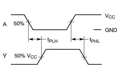
Figure 3. Switching Waveforms
