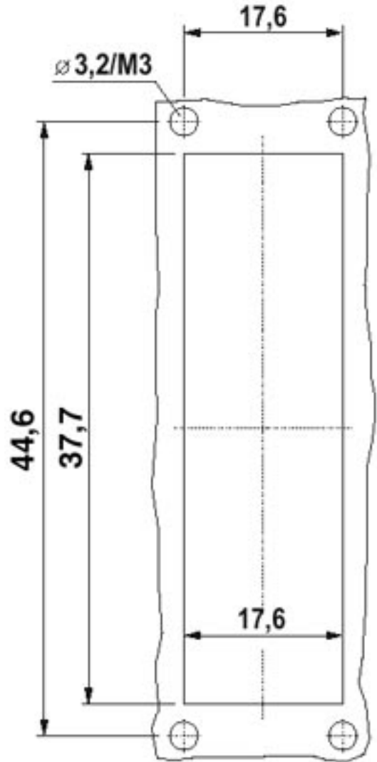
Dimensioned drawing
