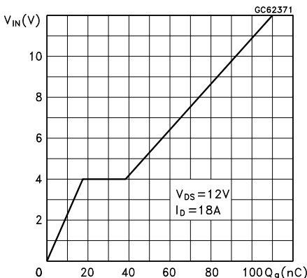
Figure 15. Input charge vs input voltage
