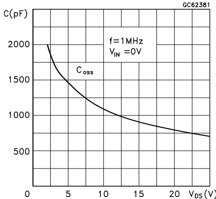
Figure 19. Capacitance variations
