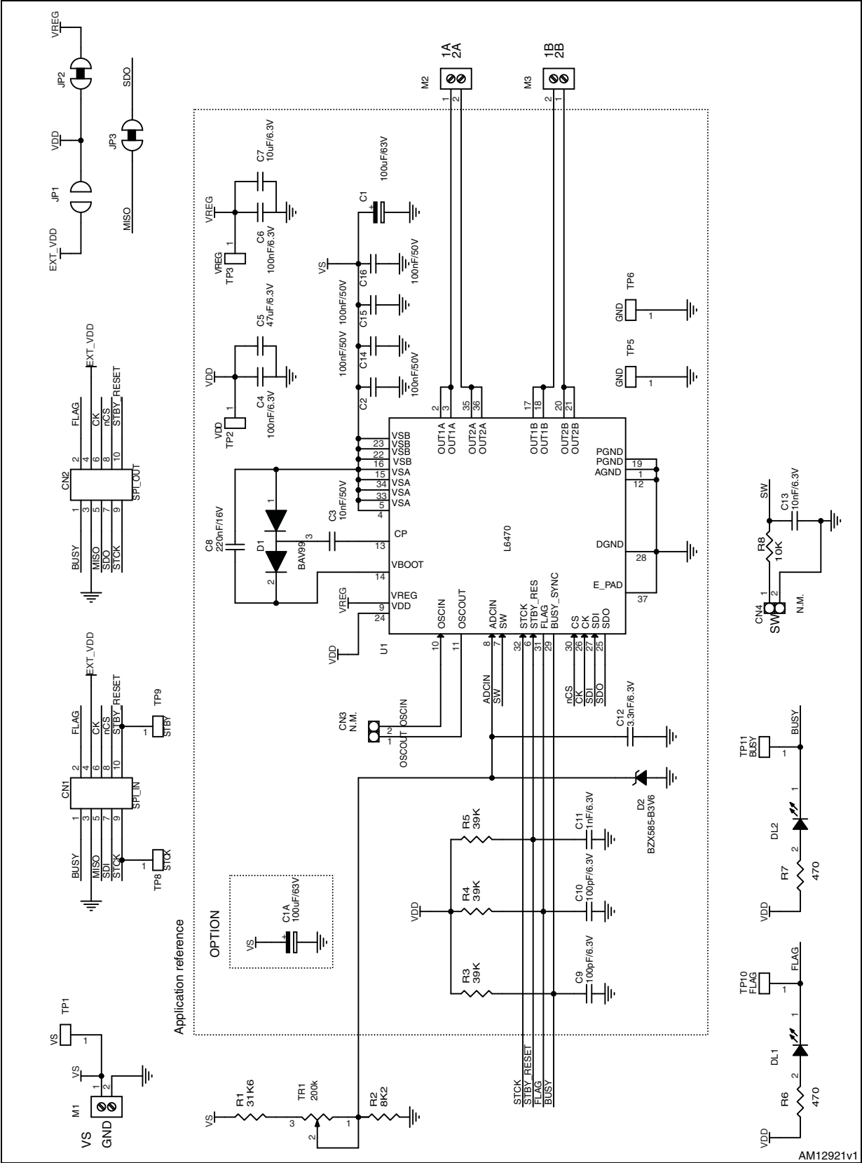
Figure 2. EVAL6470PD - schematic
