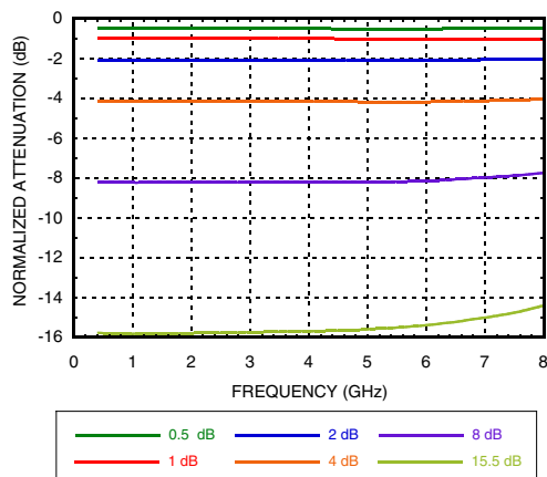
Normalized Attenuation
