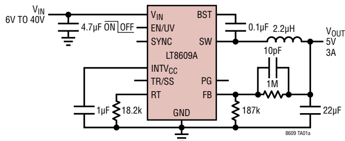
5V, 2MHz Step-Down
