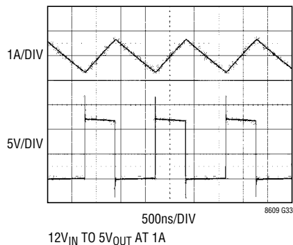
Switching Waveforms
