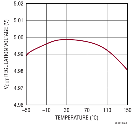
LT8609A-5 V OUT Voltage
