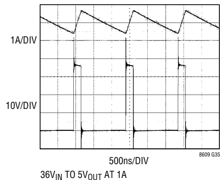
Switching Waveforms
