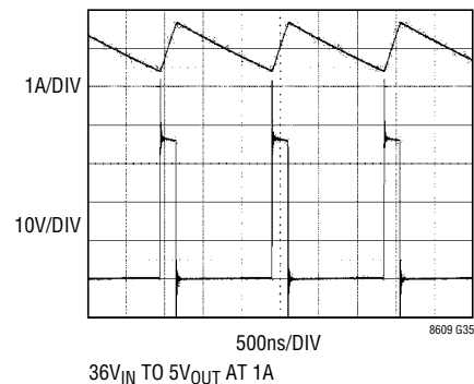
Switching Waveforms
