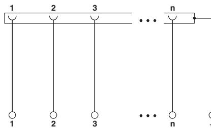
Universal circuit diagram
